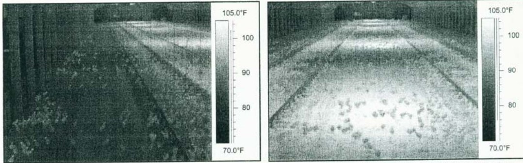
Figure 14. Side wall in house with radiant tube brooders Figure 15. Center of house with radiant tube brooders
