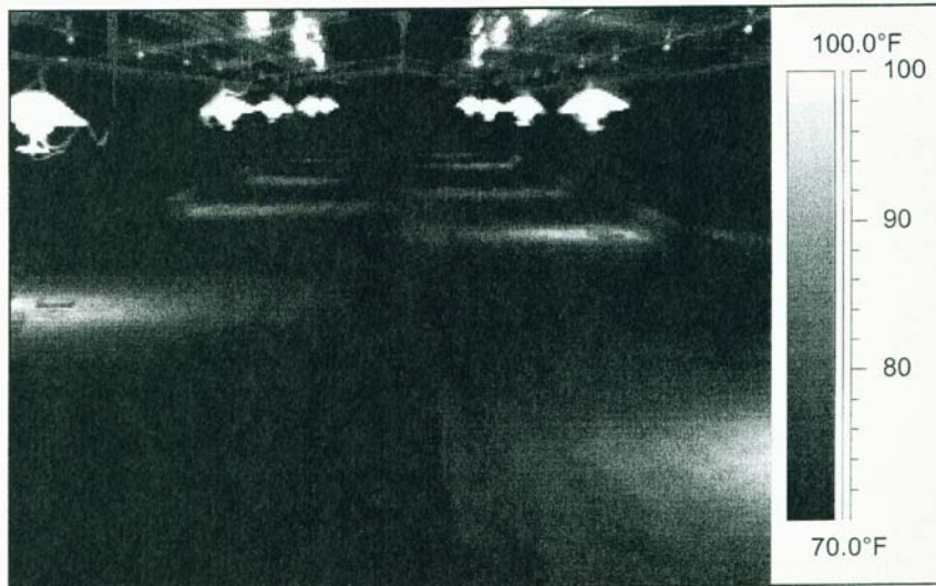
Figure 22. Insufficient gas pressure in house with radiant brooders on a 25°F morning.
