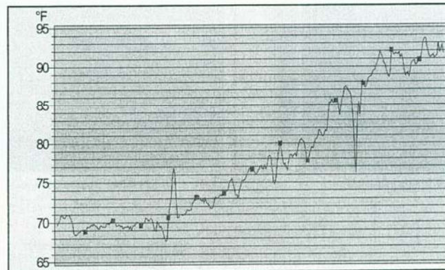
Figure 3. Floor temperatures along blue line in Figure 2.
