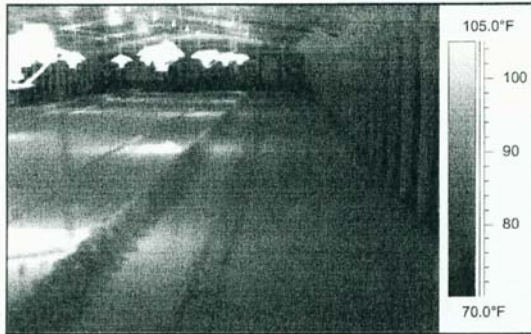
Figure 6. Side wall floor temperatures.
