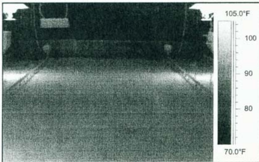
Figure 18. Paired radiant brooders near brooding curtain.
